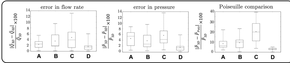
FIGURE 12. I. Pediatric surgery models and their time-varying inflow waveforms. II. Errors of mean flow rate (left) and pressure (middle) between DLP model ( \bar{Q}_{0D} , \bar{P}_{0D} ) and CFD simulation ( \bar{Q}_{3D} , \bar{P}_{3D} ) at inlets and outlets of each model. Right panel are errors of baseline Poiseuille resistance DLP ( \bar{P}_{Poiss} ).
